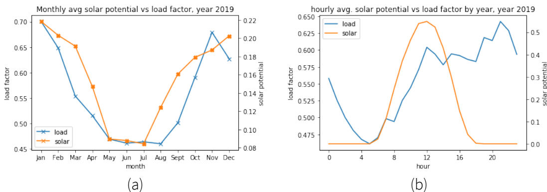
Figure 5. Solar CF compares to national electric load (a) monthly average (b) daily profile
