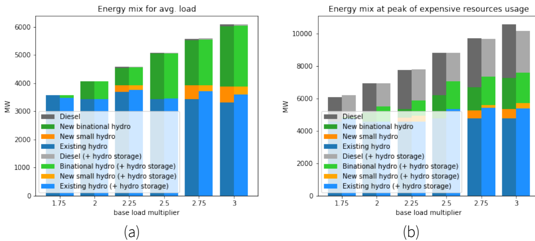
Figure 14. Comparison of energy dispatch with and without hydro storage for new hydropower plants as demand growing. (a) annual average values; (b) annual peak load hour values.
