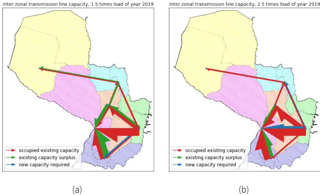
Figure 12 Major inter-zonal transmission line capacity and usage at (a) 1.5 times load of year 2019, (b) 2.5 times load of year 2019. line width is proportional to transmission capacity
