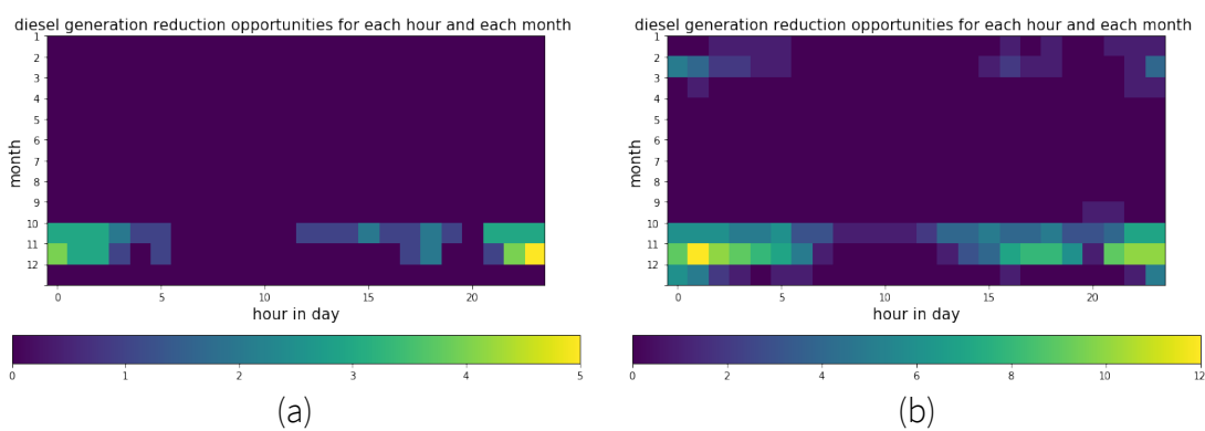
Figure 20. Number of DR event hours at each time slot each month, for (a) 1000 MW and (b) 2000 MW peak load reduction program
