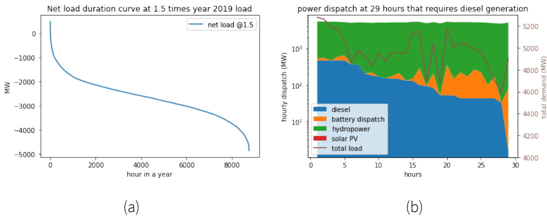
Figure 19. (a) Net load duration curve at 1.5 times year 2019 load. (b) Power dispatch at imbalance hours by source. Note: net load is defined as total load minus the generation potential of existing hydropower plants.
