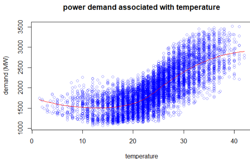
Figure AX-E1. SIN load associated with outdoor temperature for each hour in year 2019
