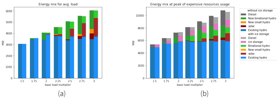
Figure 16. Comparison of energy dispatch with (right bar) and without (left bar) ice storage for future residential buildings (without showing charge of batteries or ice storage). (a) annual average values; (b) annual peak load hour values
