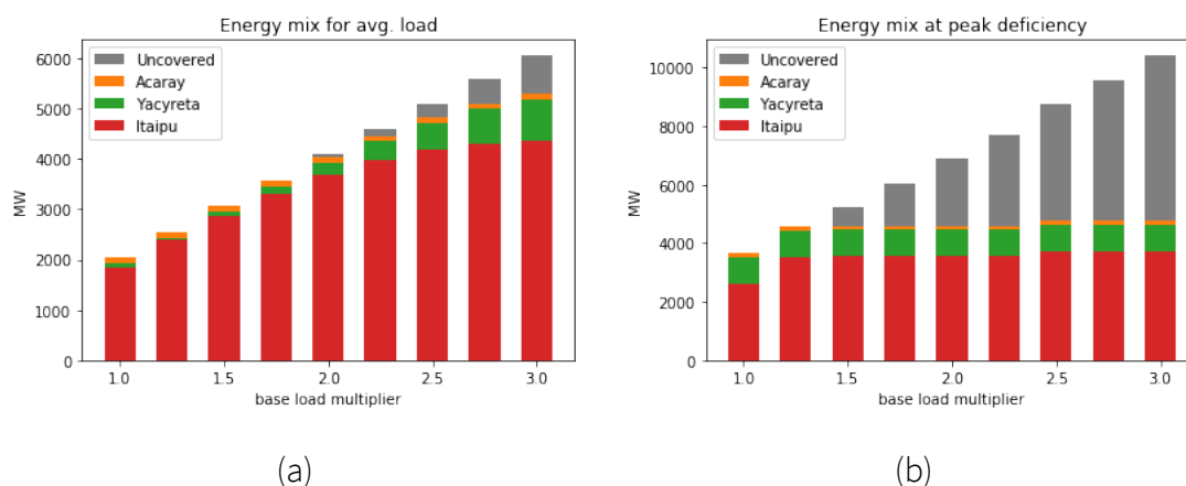
Figure 9. Current hydropower generation and the energy deficiency with the power load growth. (a): the annual average energy usage. (b): the energy usage at the peak load hour.
