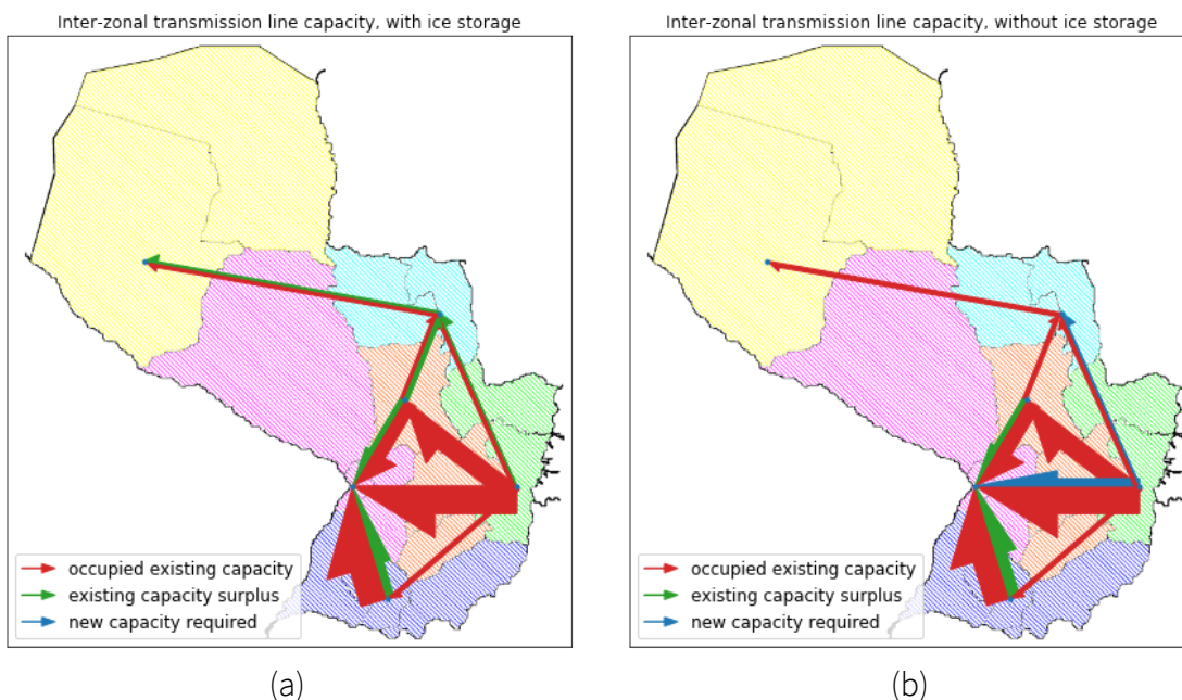
Figure 17. Interzonal transmission usage comparison between with and without ice storage, at 2.5 times electric load of year 2019
