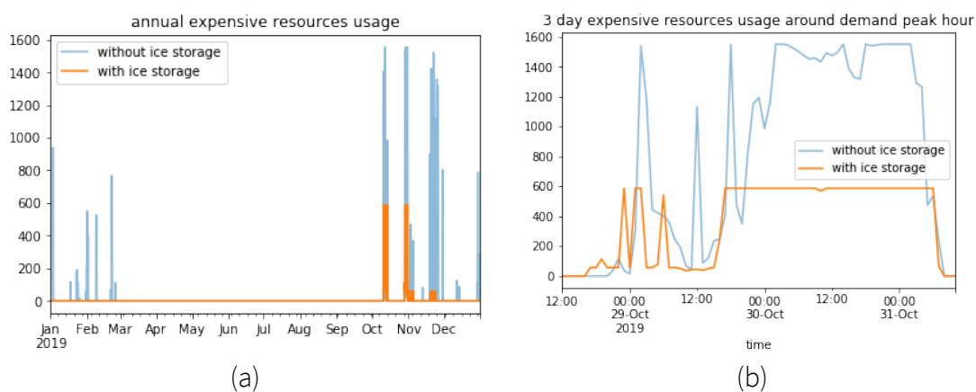
Figure 18. Expensive dispatchable resources usage with and without ice storage. load at 2.5 times year 2019 load (a) annually; (b) three days peak usage window
