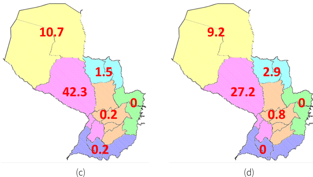
Figure 15. geographical distribution of average usage of expensive dispatchable resources (unit: MW) with and without hydro storage. (a) and (b) are at 2 times year 2019 load, (c) and (d) are at 3 times year 2019 load. Whereas (a) and (c) without any storage, (b) and (d) allows hydro storage for new hydropower plants
