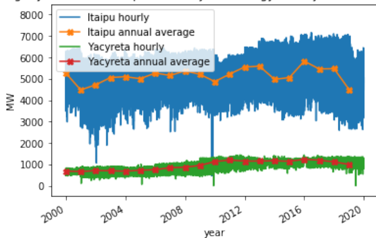
Paraguayan share of Itaipu and Yacyreta energy, hourly and annual average
