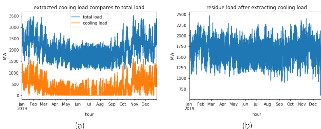
Figure 8. Simulated cooling load compares to SIN total load and residual load
