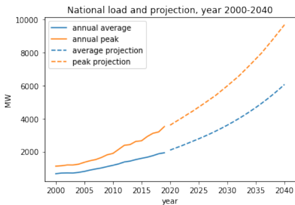
Figure 6. Annual average and peak load growth projection by ANDE, under 'optimistic scenario'.
