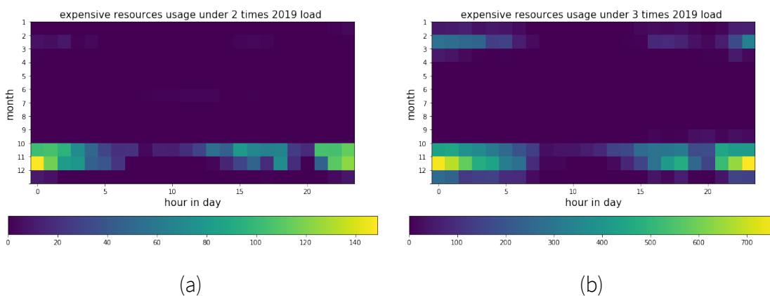
Figure 11. The usage expensive resources electricity generation in time domain, unit: MW. (a) doubled 2019 demand; (b) tripled 2019 demand.
